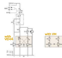
AC or DC remote control
