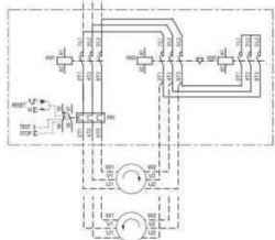
Star-delta starters Power circuit
